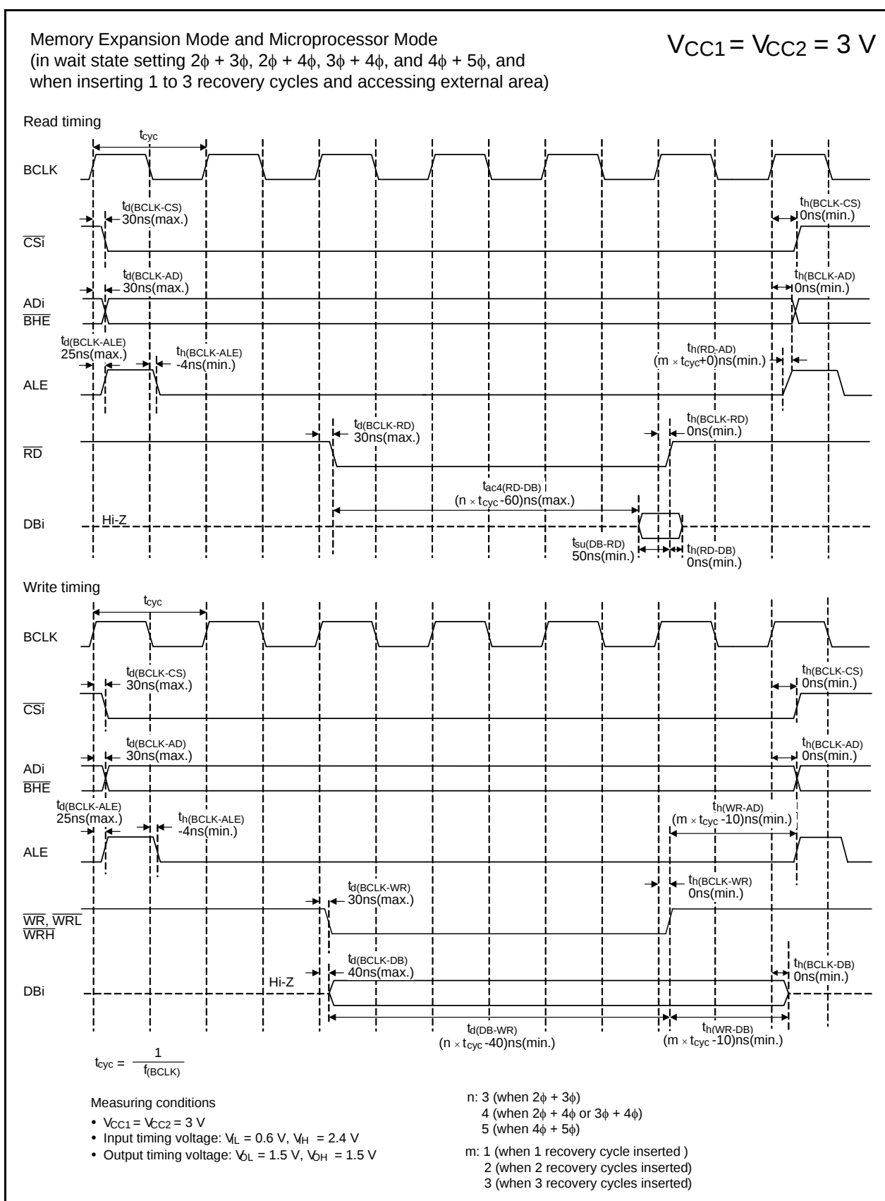
Figure 5.32 Timing Diagram
