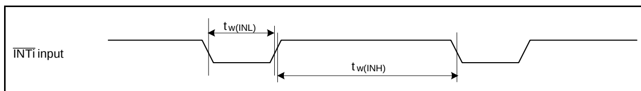
Figure 5.25 External Interrupt \overline{\text{INTi}} Input
