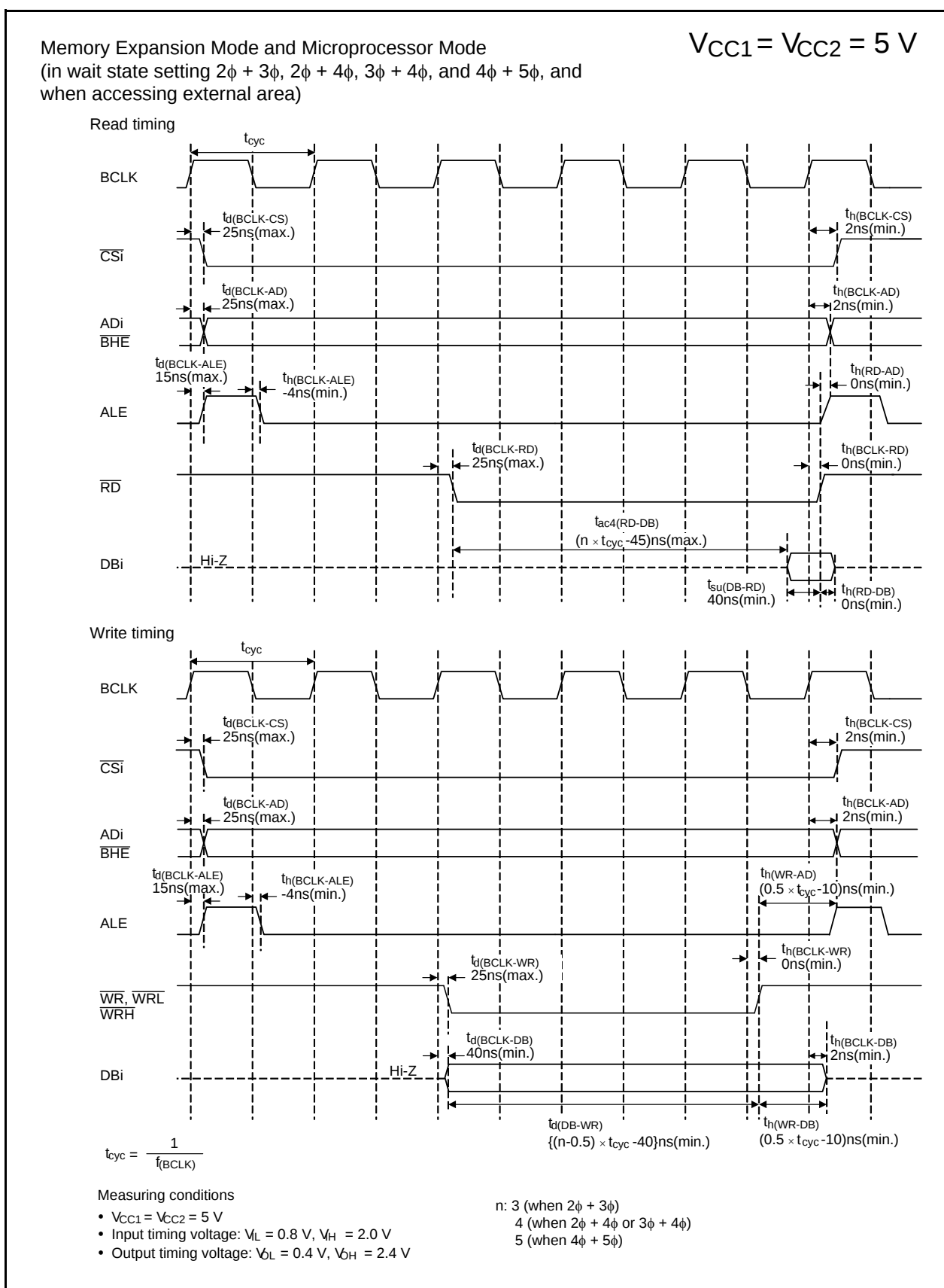
Figure 5.17 Timing Diagram
