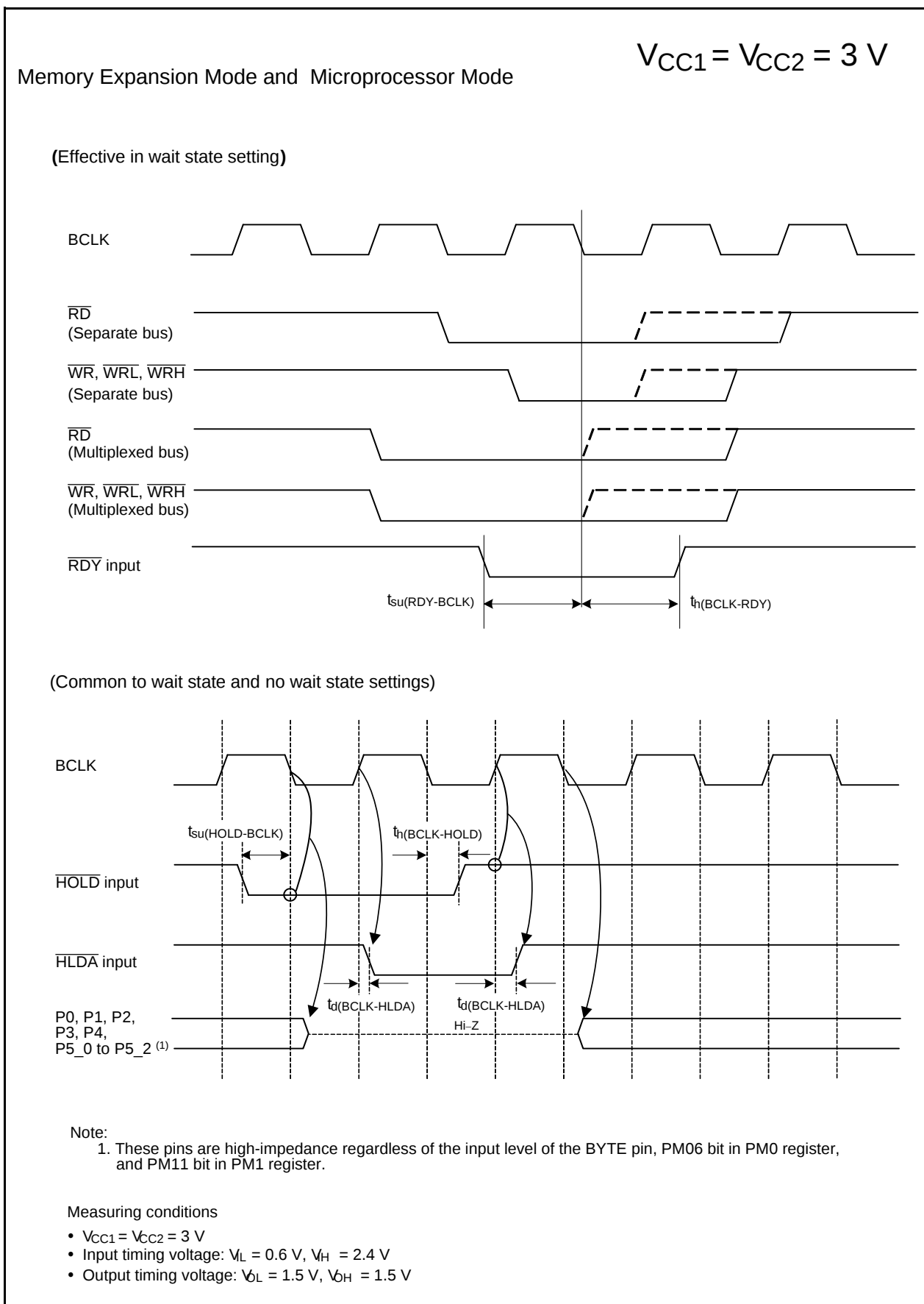
Figure 5.26 Timing Diagram
