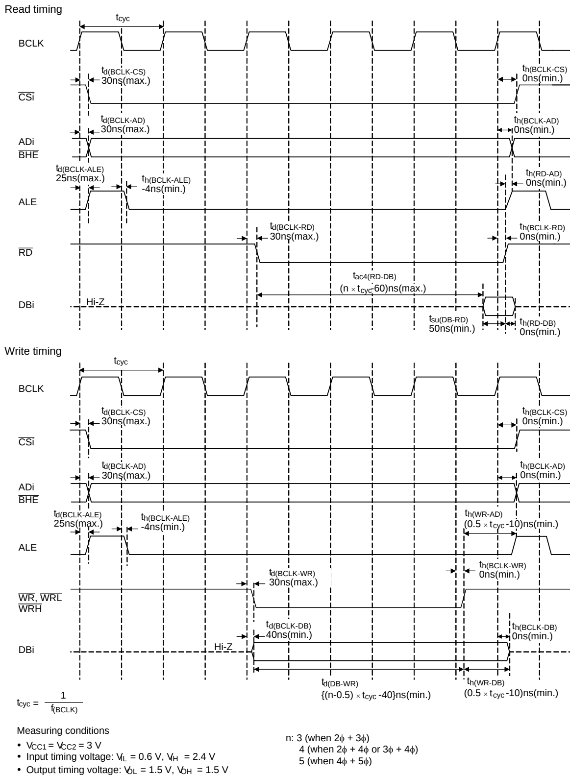
Figure 5.31 Timing Diagram
