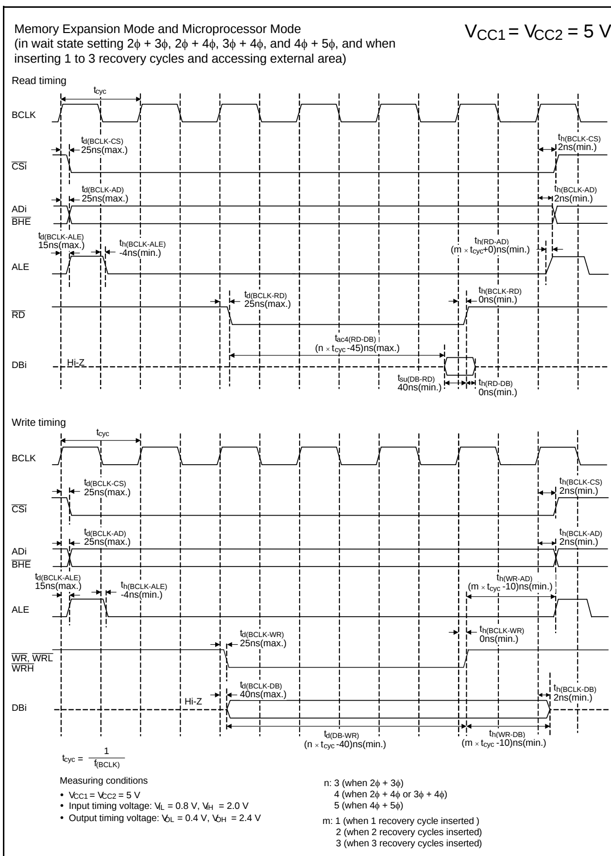
Figure 5.18 Timing Diagram
