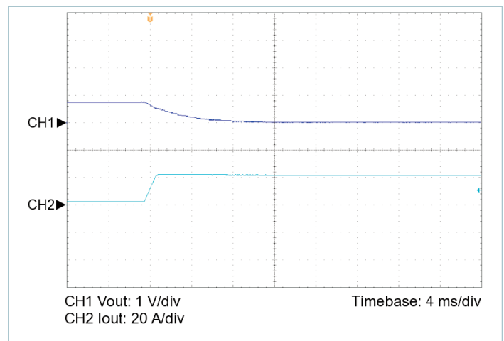
Figure 8 — 10% to 100% load transient response, V_{IN} = 28\text{ V} , nominal trim, C_{OUT\_EXT} = 680\text{ }\mu\text{F}
