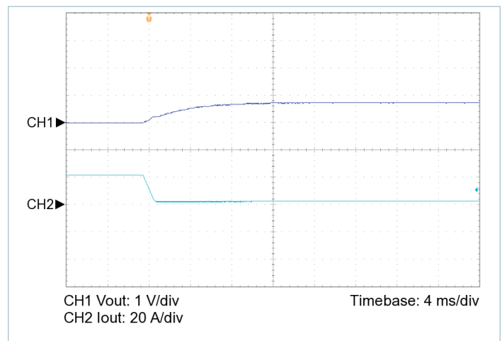
Figure 7 — 100% to 10% load transient response, V_{IN} = 28\text{ V} , nominal trim, C_{OUT\_EXT} = 680\text{ }\mu\text{F}
