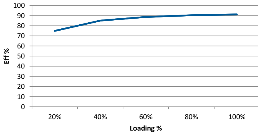
AM2D-1215S-RZ Efficiency vs. Loading
