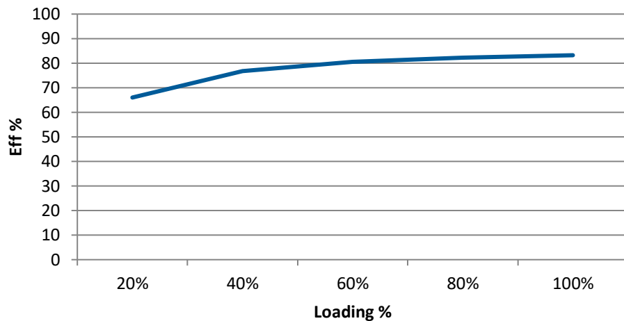
AM2D-0505S-RZ Efficiency vs. Loading
