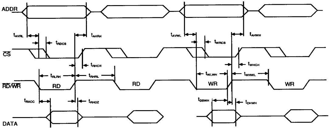
Figure 25. Microprocessor Read/Write Timing
