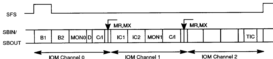
Figure 7. IOM-2 Terminal Mode Frame Structure
