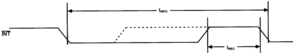
Figure 26. \overline{INT} Timing
