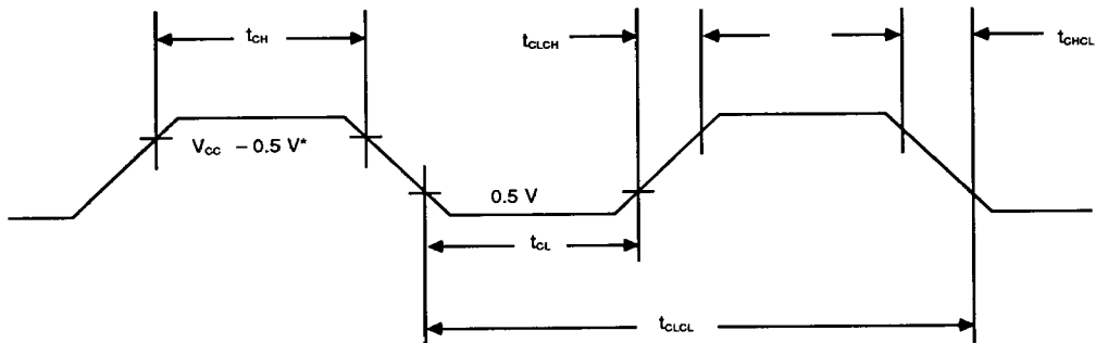
Figure 29. External Clock Driver (XTAL 2 ) Timing
