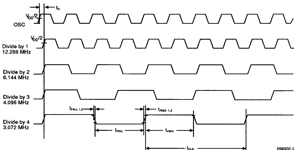
Figure 30. OSC/MCLK Timing
