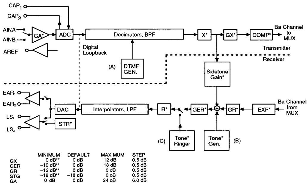
Figure 3. Main Audio Processor Block Diagram
