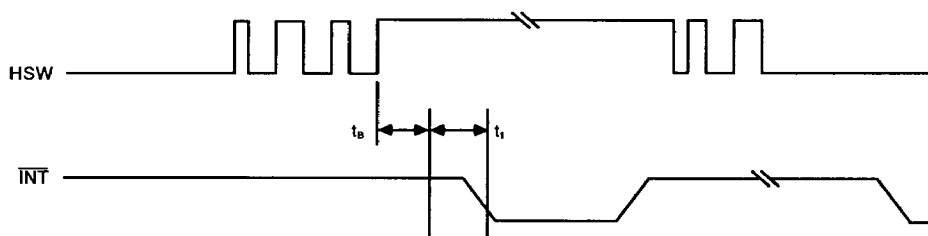
Figure 28. Hookswitch Debounce Timing
