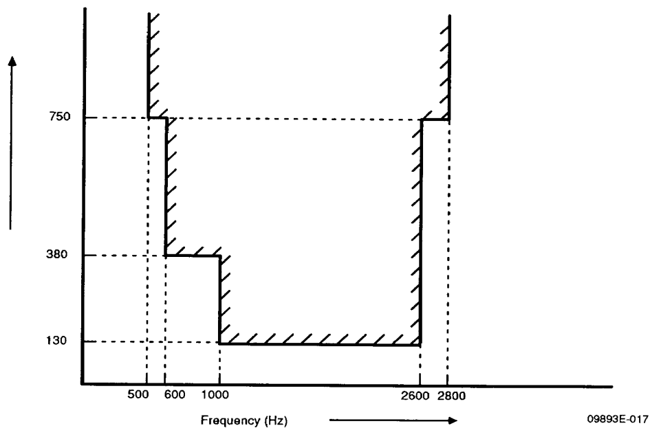
Figure 14. Group Delay Variation with Frequency (Transmit)
