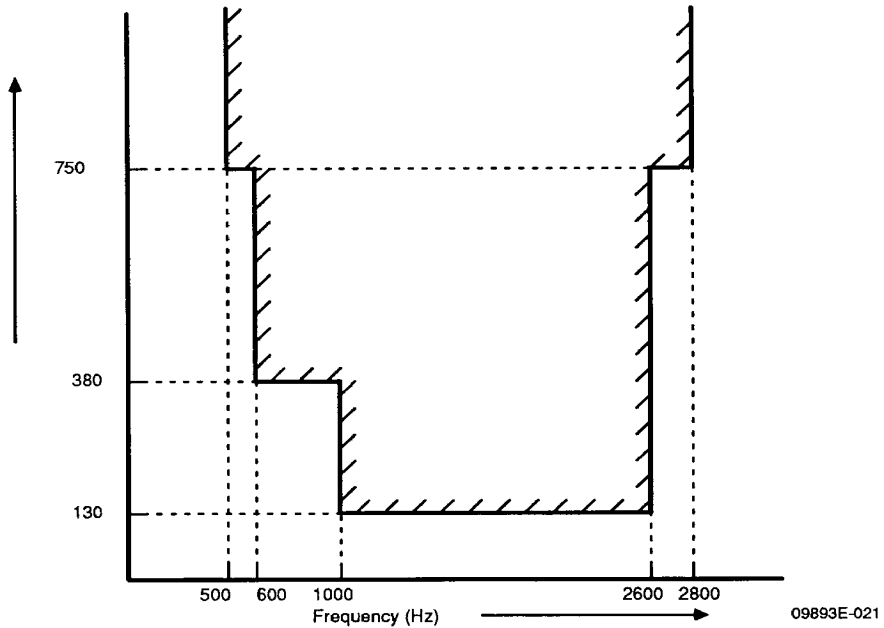
Figure 18. Group Delay Variation with Frequency (Receive)
