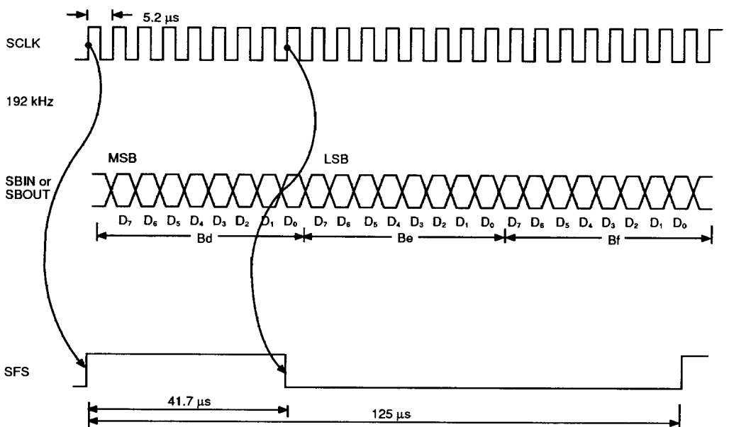
Figure 6. Serial Bus Port Mode Timing
