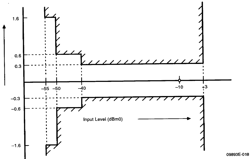
Figure 15. Gain Tracking Error (Transmit) (CCITT Method 2 at 1020 Hz)
