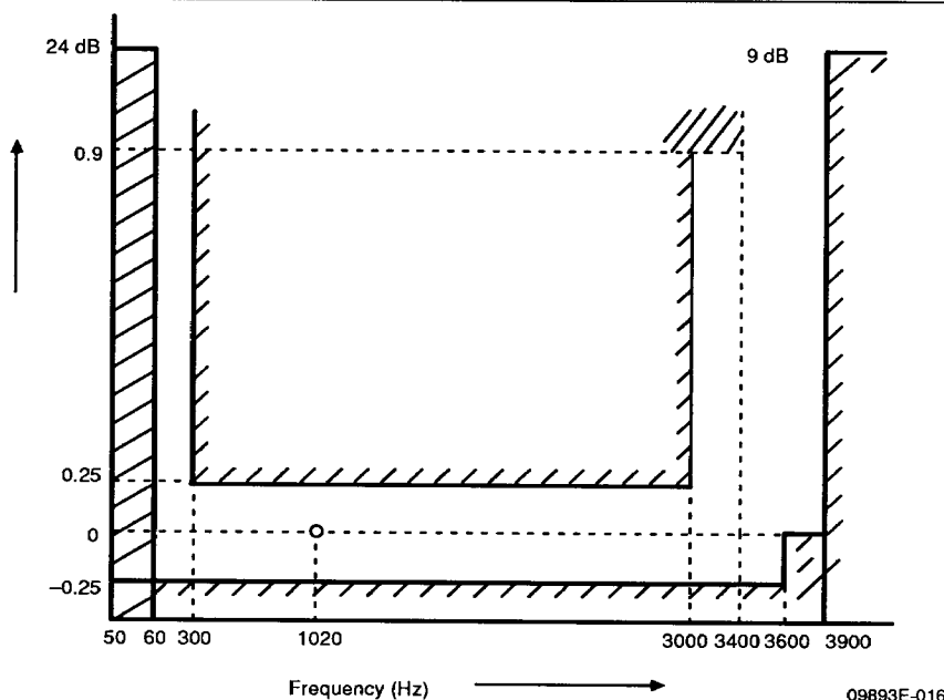
Figure 13. Attenuation/Frequency Distortion (Transmit)
