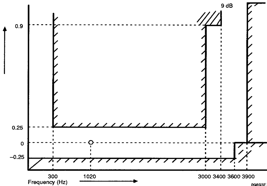
Figure 17. Attenuation/Frequency Distortion (Receive)
