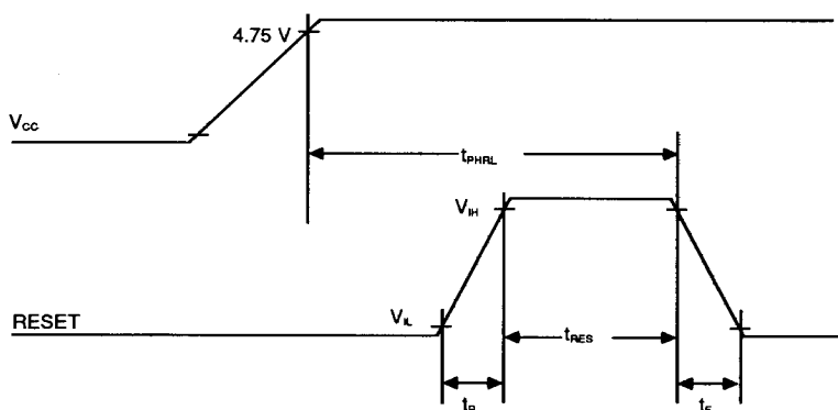
Figure 27. Reset Timing
