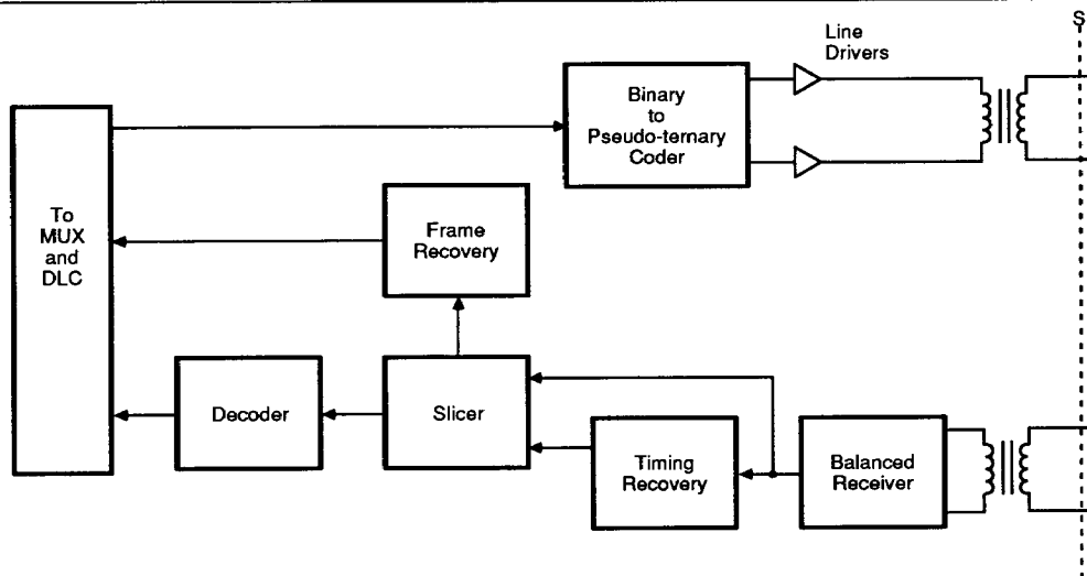
Figure 1. LIU Block Diagram
