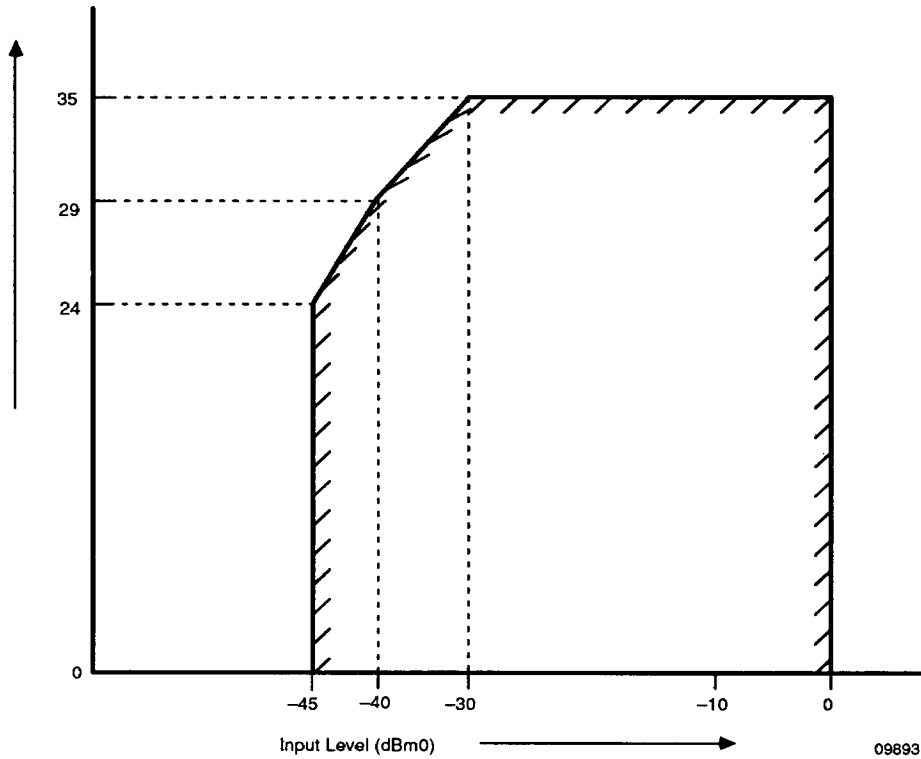
Figure 20. Signal to Total Distortion Ratio (Receive) (CCITT Method 2 at 1020 Hz)
