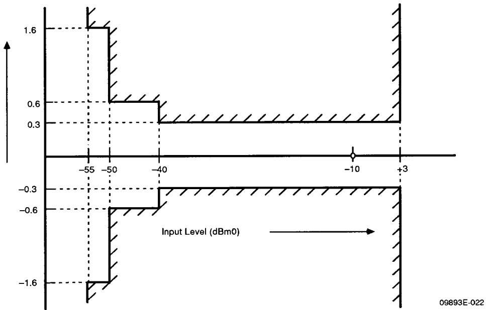
Figure 19. Gain Tracking Error (Receive) (CCITT Method 2 at 1020 Hz)
