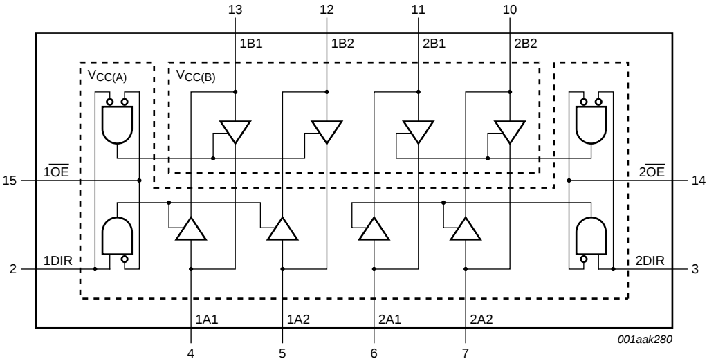
Fig 1. Logic symbol
