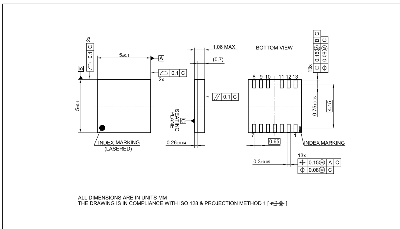
Figure 21 PG-TFLGA-13-1 outline
