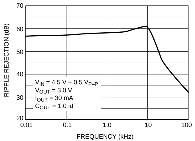
Figure 7. Ripple Rejection/Frequency
