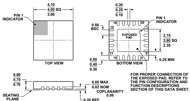
Figure 32. 20-Lead Lead Frame Chip Scale Package [LFCSP_WQ] 4 mm × 4 mm Body, Very, Very Thin Quad (CP-20-8)
