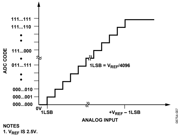
Figure 23. Straight Binary Transfer Characteristic
