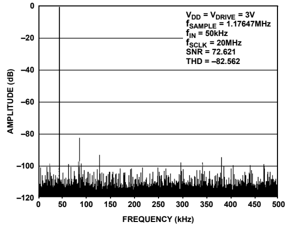
Figure 3. Typical FFT
