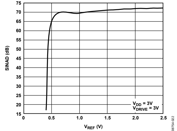
Figure 14. SINAD vs. Reference Voltage
