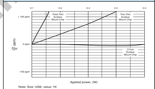
FIGURE 8 - BEHAVIOR OF THREE DIFFERENT RESISTOR TECHNOLOGIES UNDER APPLIED POWER (POWER COEFFICIENT TEST)
