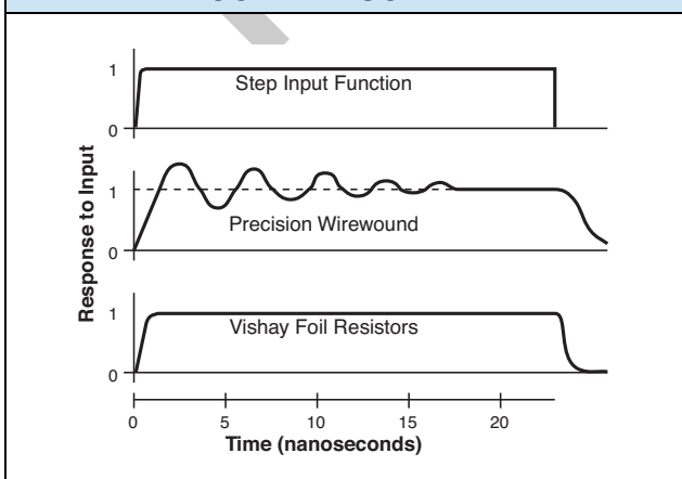
FIGURE 7 - PULSE RESPONSE COMPARISON
