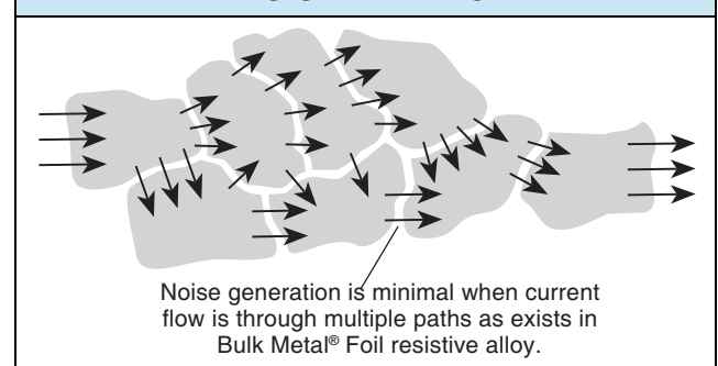
FIGURE 9 - CURRENT PATH IN A RESISTIVE ALLOY
