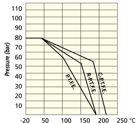
Pressure - Temperature Diagram
