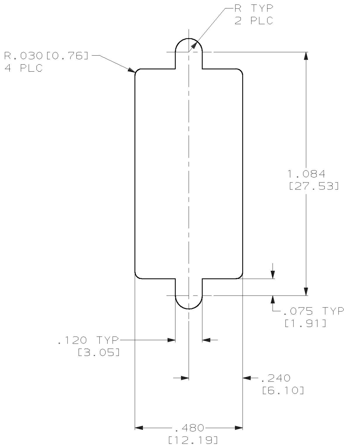
SUGGESTED PANEL CUTOUT SCALE 4:1
