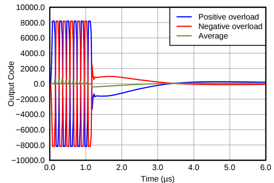
Figure 53. Pulse Inversion Asymmetrical Positive Input
