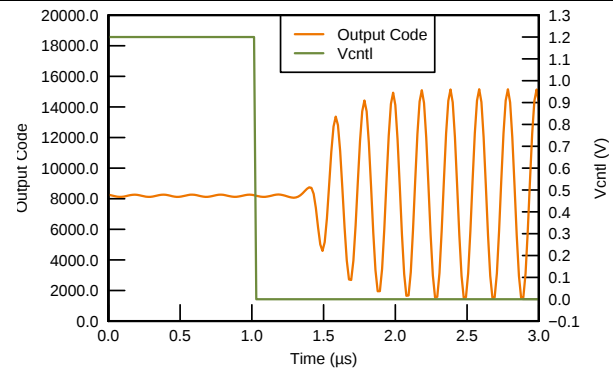
Figure 51. VCNTL Response Time
