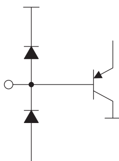
Figure 72. Equivalent Circuits of V_{\text{CNTLP/M}}
