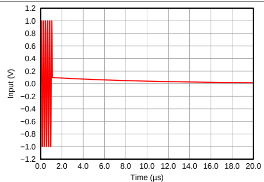
Figure 51. VCNTL Response Time
