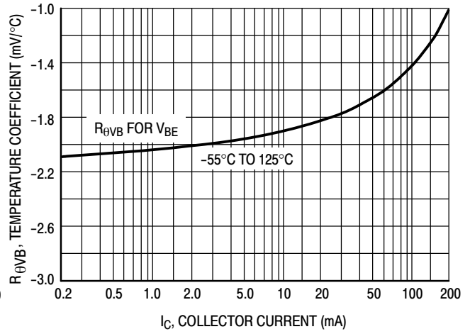
Figure 18. Base-Emitter Temperature Coefficient
