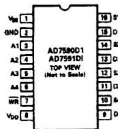
16-Pin DIP
