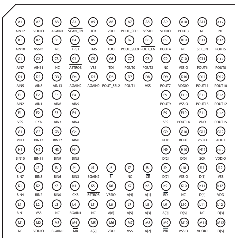
Figure 3. CLC5903SM FBGA Pinout
