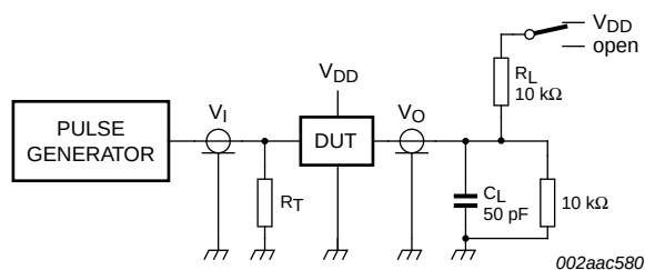
Fig 14. Test circuitry for enable/disable times, SDOUT ( t_{\text{en}}(\text{SDOUT}) and t_{\text{dis}}(\text{SDOUT}) )
