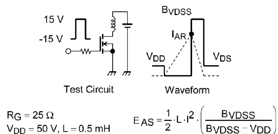
Fig. 8.16 Test Circuit/Waveform
