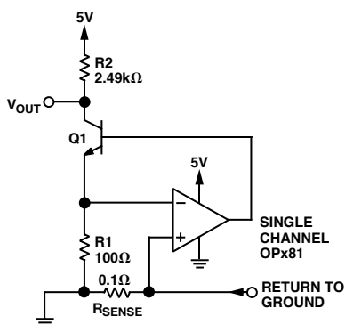
Figure 7. Low-Side Load Current Monitor
