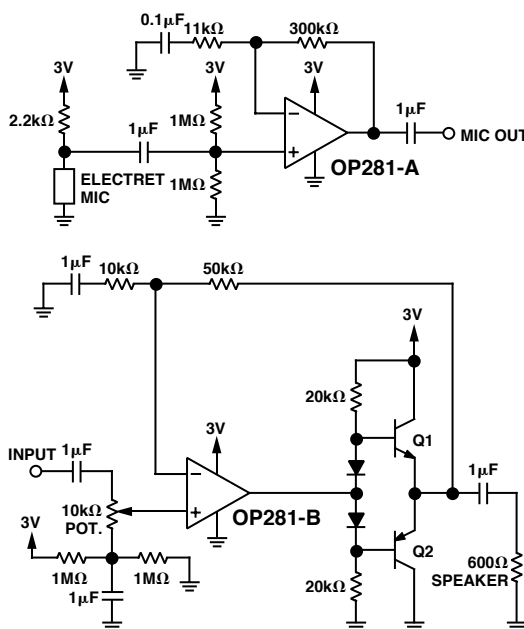
Figure 10. Two-Way Amplifier in a Battery-Powered Telephone Headset
