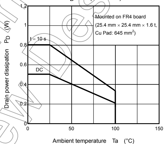
P_D - T_a (MOSFET)
