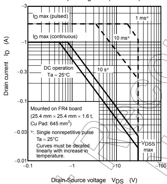
Safe operating area (MOSFET)
