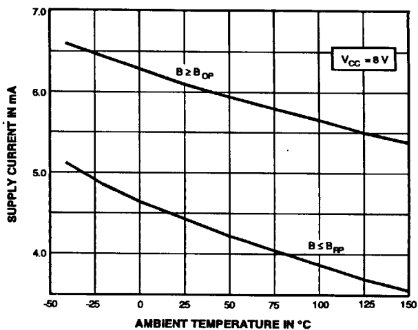
SUPPLY CURRENT
