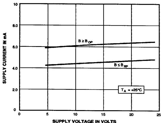
SUPPLY CURRENT
