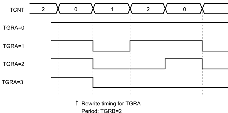
Figure 14.13 Examples of PWM Mode Operation (2)
