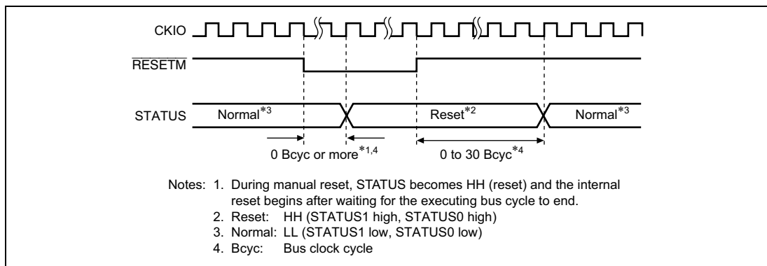
Figure 11.3 Manual Reset STATUS Output
