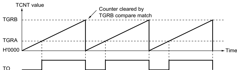
Figure 14.12 Example of PWM Mode Operation (1)
