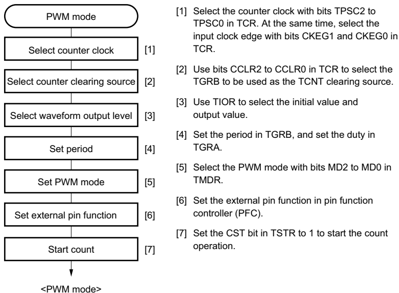
Figure 14.11 Example of PWM Mode Setting Procedure
