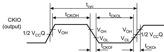
Figure 25.4 CKIO Clock Output Timing
