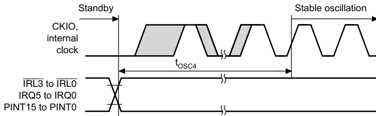
Figure 25.8 Oscillation Settling Time at Standby Return (Return by IRQ5 to IRQ0, PINT15 to PINT0, and \overline{IRL3} to \overline{IRL0} )
