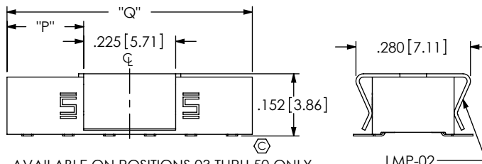
FIGURE 5 (-P: PICK & PLACE PAD)
