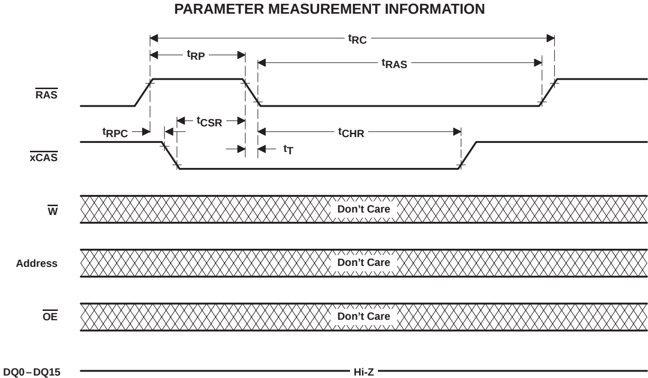
Figure 11. Automatic-CBR-Refresh-Cycle Timing
