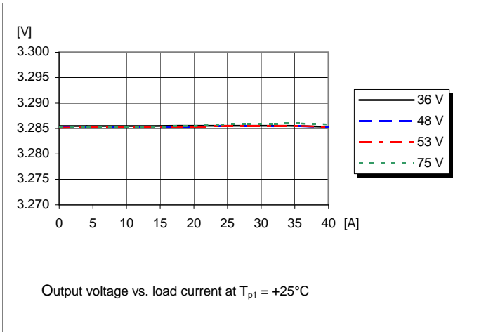
Output Characteristics
