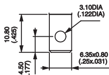
Sold.lug/Quick-conn.
