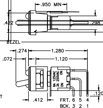
J95—TWO LED's
