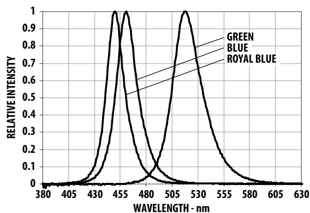
Figure 12. Relative Intensity vs. Wavelength for Blue and Green
