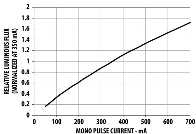
Figure 13. Relative Luminous Flux vs. Mono Pulse Current
