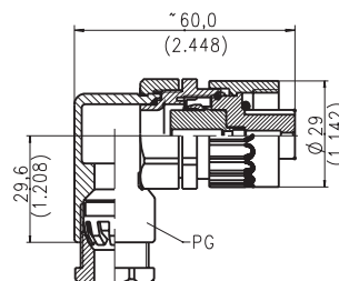
Typical right angle Plug dimensions
