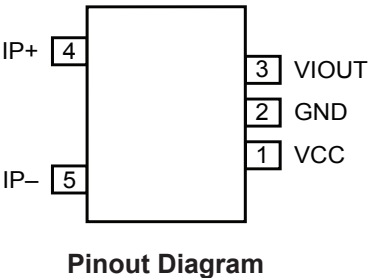
Pinout Diagram
