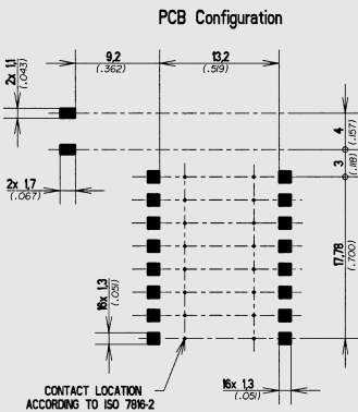
CCM04-5004*/1201/1202/1203/1204 PCB Layout
