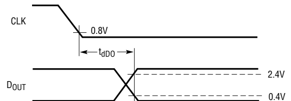
Voltage Waveforms for D_{OUT} Delay Time, t_{dD}
