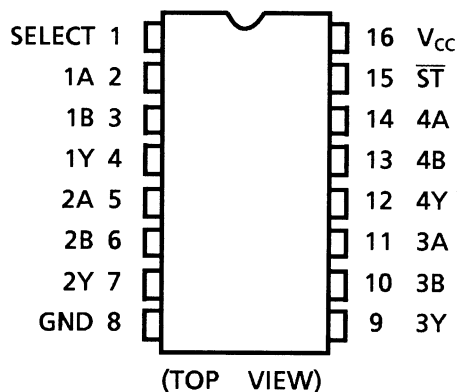
TC74HC157A
