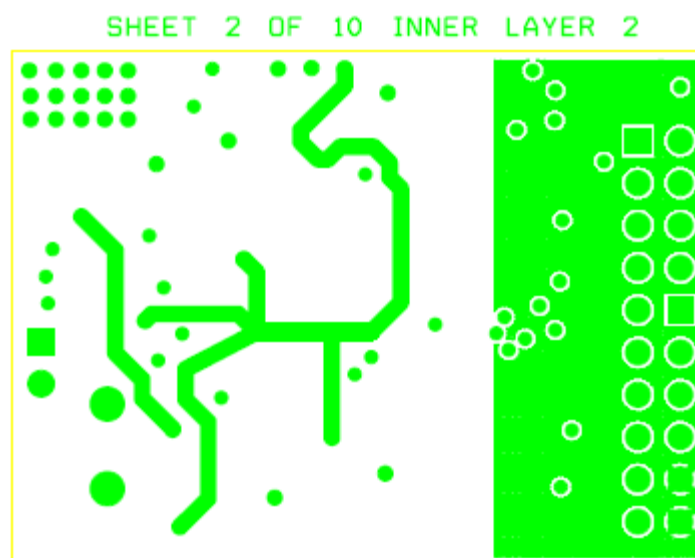
Figure 6: 73M1866B Keychain Demo Board Ground Inner Layer
