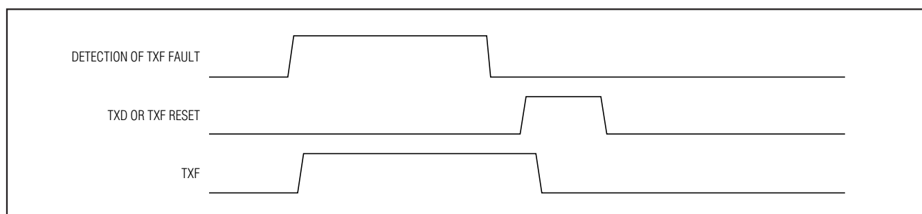
Figure 15b. TXF Latched Operation
