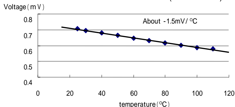
TH-out characteristic (for reference)
