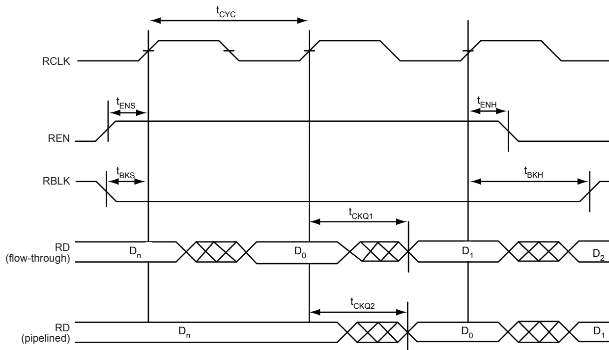
Figure 2-32 • FIFO Read
