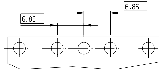
LAYOUT DIMENSIONS (after plating) CONNECTOR SIDE VIEW
