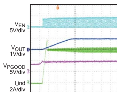
PGOOD, Startup Through EN
