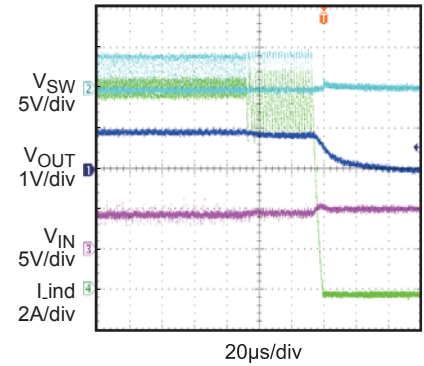
Over-current Protection
