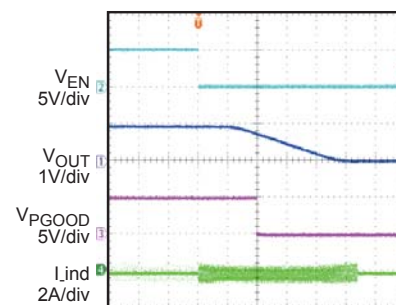
PGOOD, Shutdown Through EN
