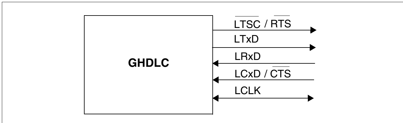
Figure 47 GHDLC Interface Lines
