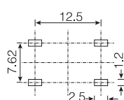
PCB Layout (SMD)
