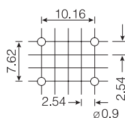
PCB Layout (through-hole)
