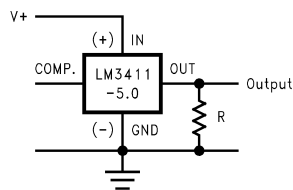
Figure 34. Voltage Detector
