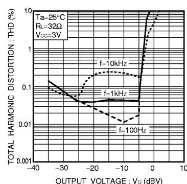
Fig.8 Total harmonic distortion vs. output voltage (II)
