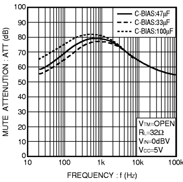
Fig.12 MUTE attenuation vs. frequency
