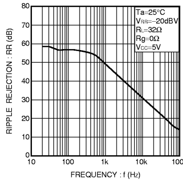
Fig.13 Ripple rejection vs. frequency
