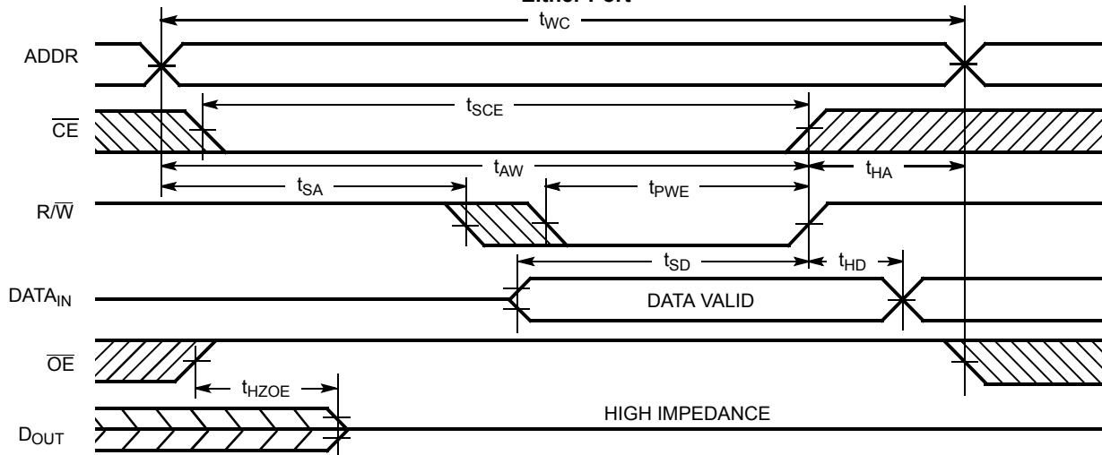
Figure 6. Write Cycle No. 1 ( \overline{\text{OE}} Three-States Data I/Os – Either Port) [30, 31]
