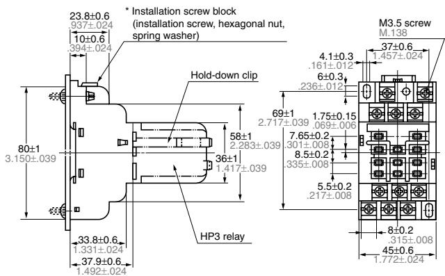
External dimensions
