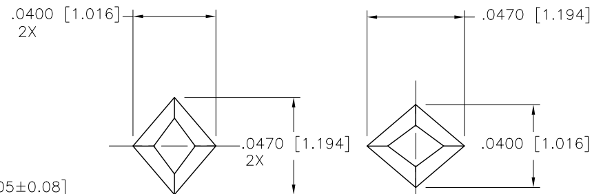
VIEW E-E SCALE 4/1
