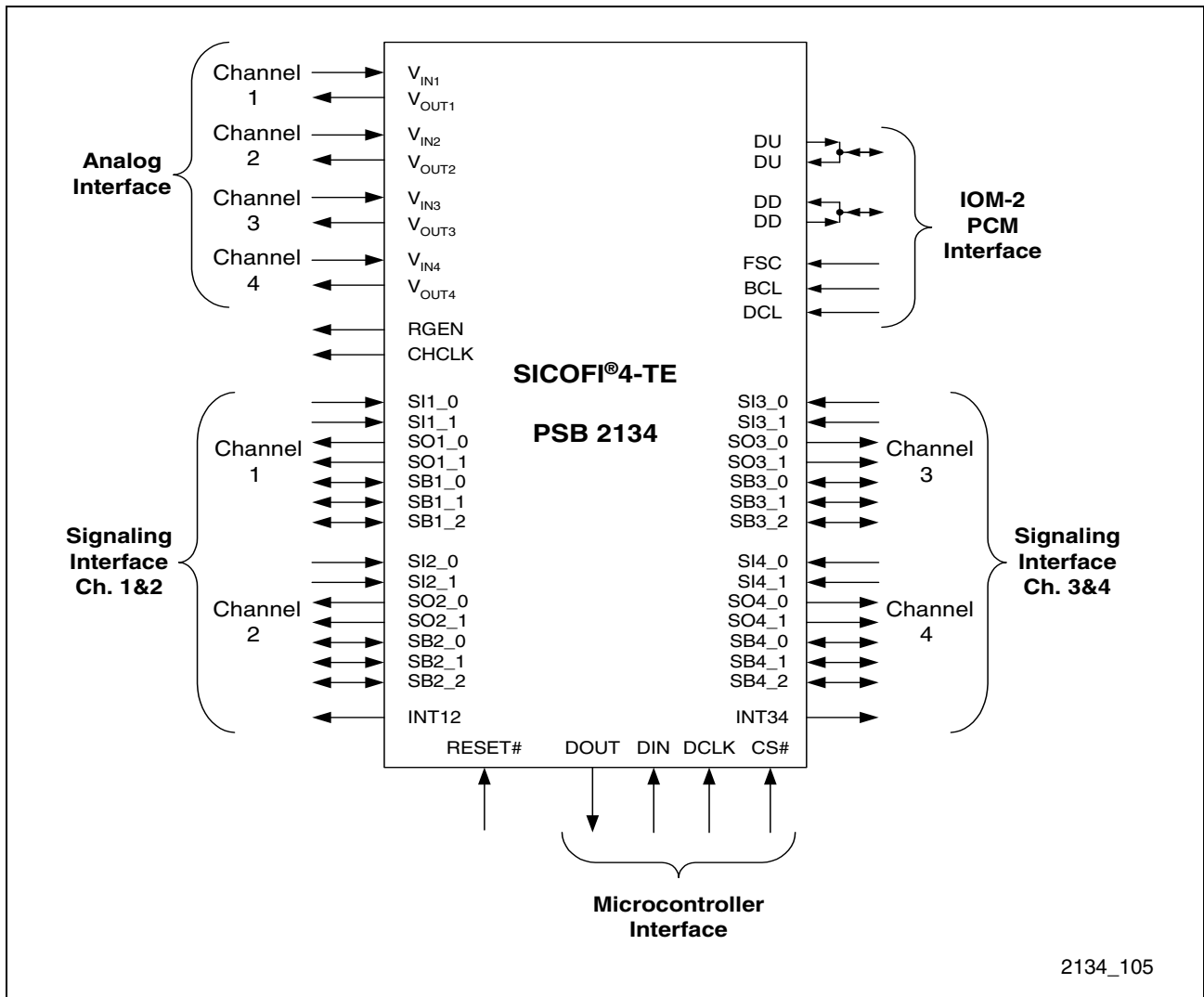
Figure 2 SICOFI®4-TE Logic Symbol
