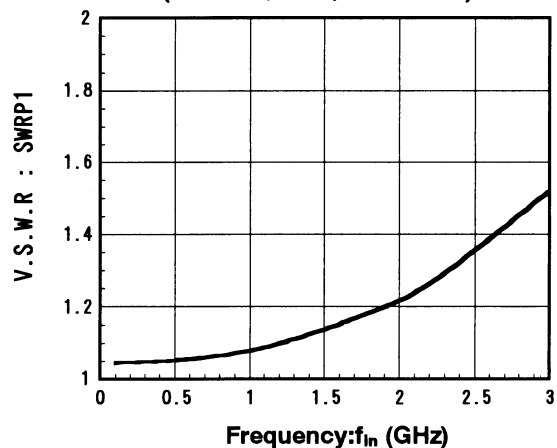
P2-PC(ON)V.S.W.R vs. Frequency ( V_{CTR}=0V/2.7V , P_{in}=0dBm )
