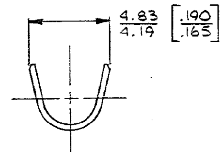
SECT B-B
