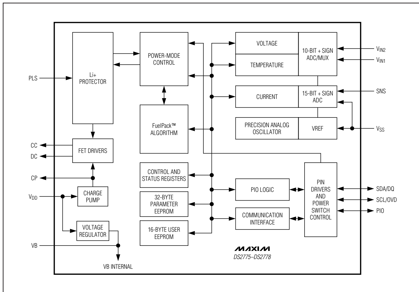
Block Diagram
