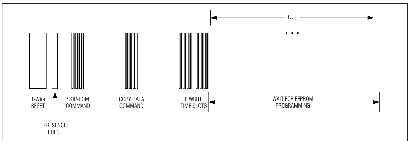
Figure 27. Copy Data Command
