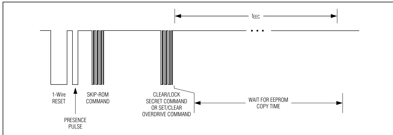
Figure 28. Clear/Lock Secret, Set/Clear Overdrive Commands
