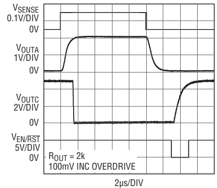
LT6108-1 Step Response
