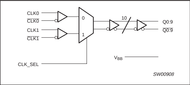
Figure 3. Logic symbol
